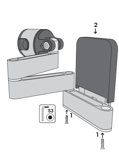
B3 Thin Mount / Adhesive
