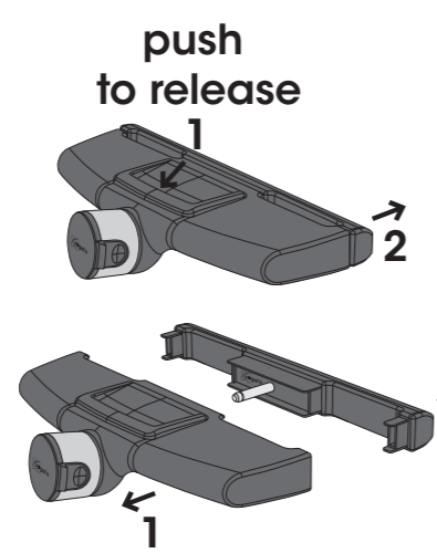
1 Car Mount
