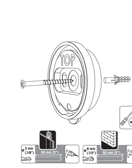
A2 Thin Mount
