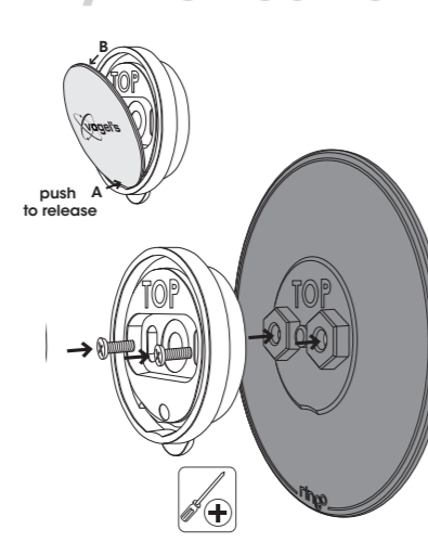
B4 Thin Mount / Adhesive
